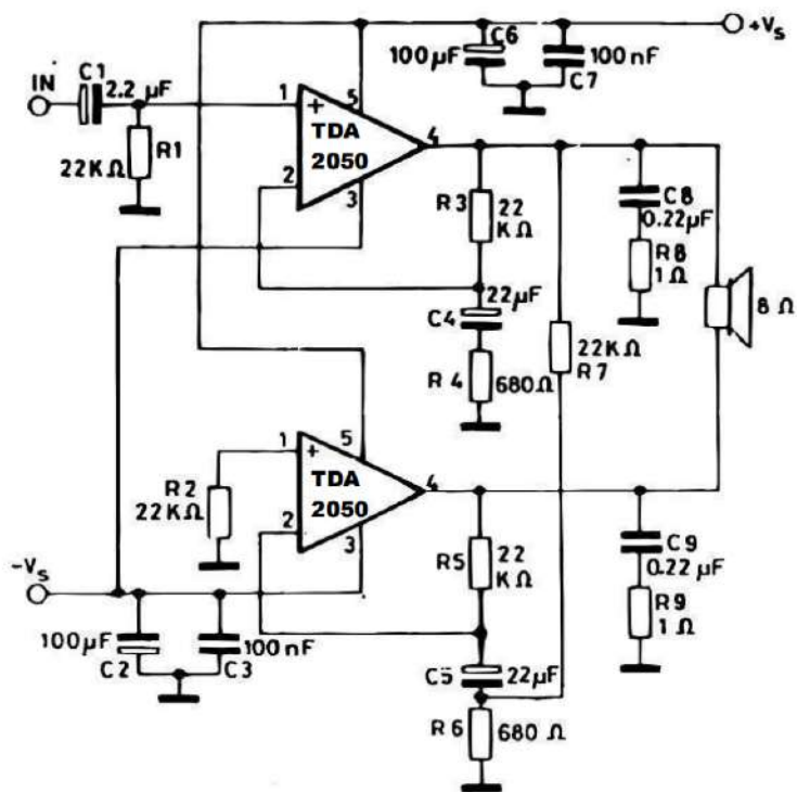
Figure 13 : Bridge Amplifier with Split Power Supply ( P_O = 34W , V_S = \pm 16V )
