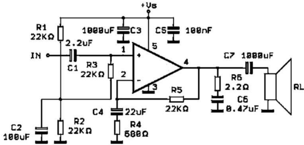
Figure 1 : Single Supply Amplifier
