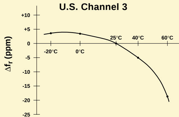
Resonant Frequency Change with Temperature KAR—61CT
