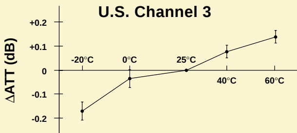
Attenuation Change at Resonance with Temperature KAR—61CT
