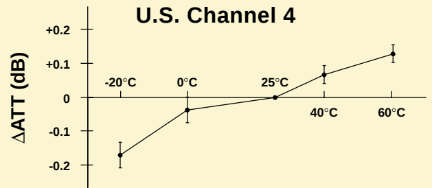
Attenuation Change at Resonance with Temperature KAR—61CT
